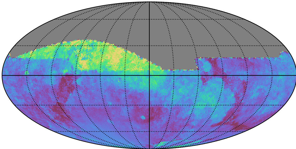
roman_v3.3_10yrs All sky all bands: Median moonDistance
