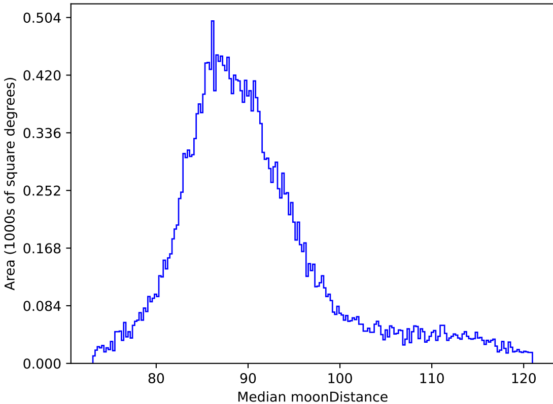
roman_v3.3_10yrs All sky all bands: Median moonDistance
