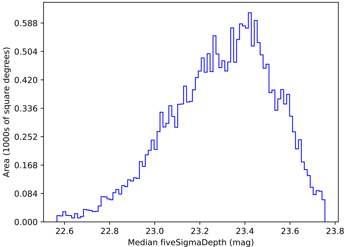
roman_v3.3_10yrs Yr 1 u band: Median fiveSigmaDepth
