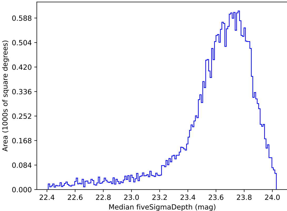
roman_v3.3_10yrs Yr 1 i band: Median fiveSigmaDepth
