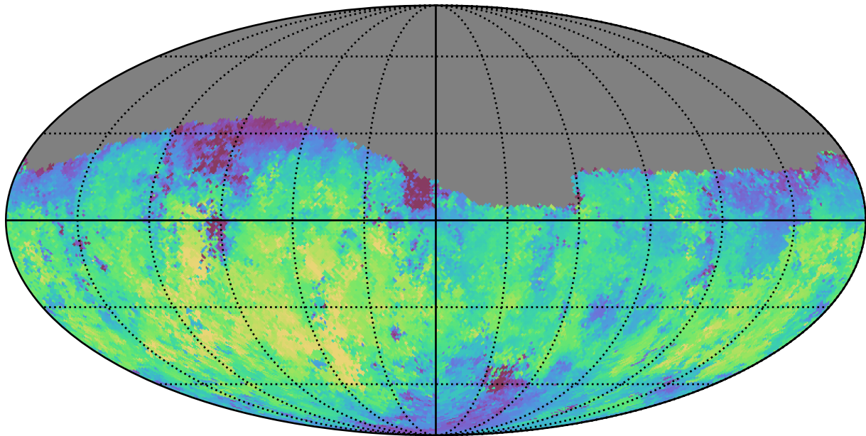
roman_v3.3_10yrs Yr 1 g band: Median fiveSigmaDepth
