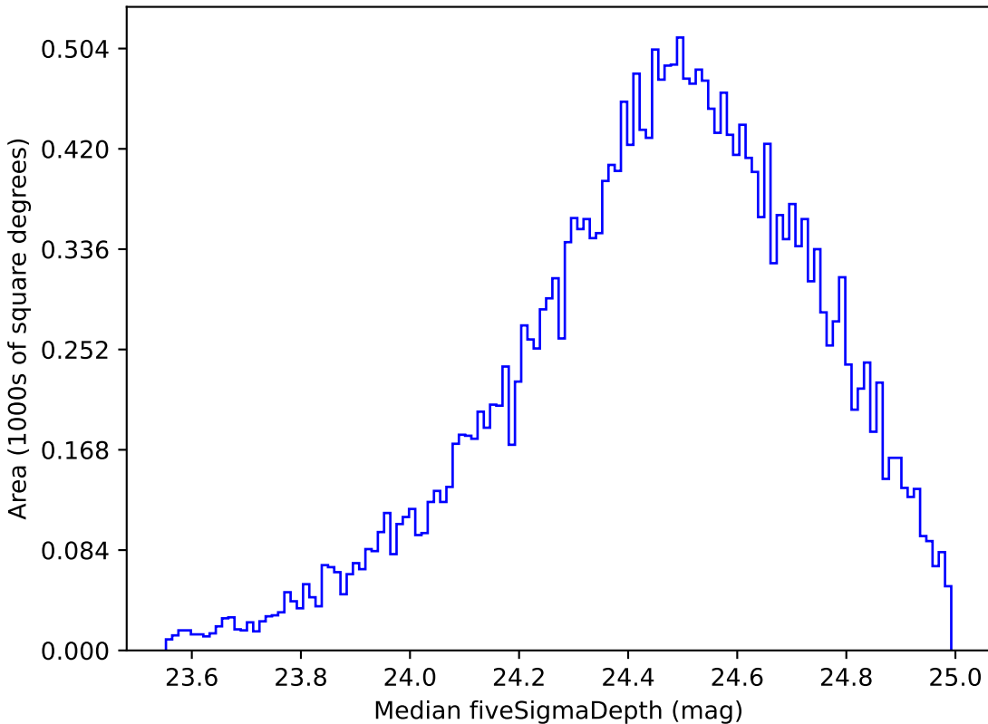
roman_v3.3_10yrs Yr 1 g band: Median fiveSigmaDepth
