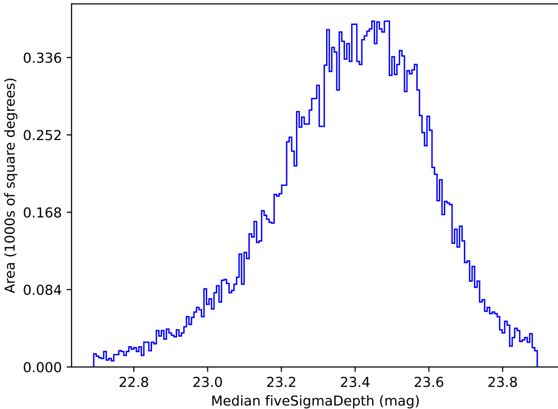
roman_v3.3_10yrs Yr 1 all bands: Median fiveSigmaDepth
