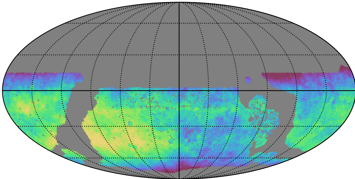
roman_v3.3_10yrs WFD z band: Median fiveSigmaDepth
