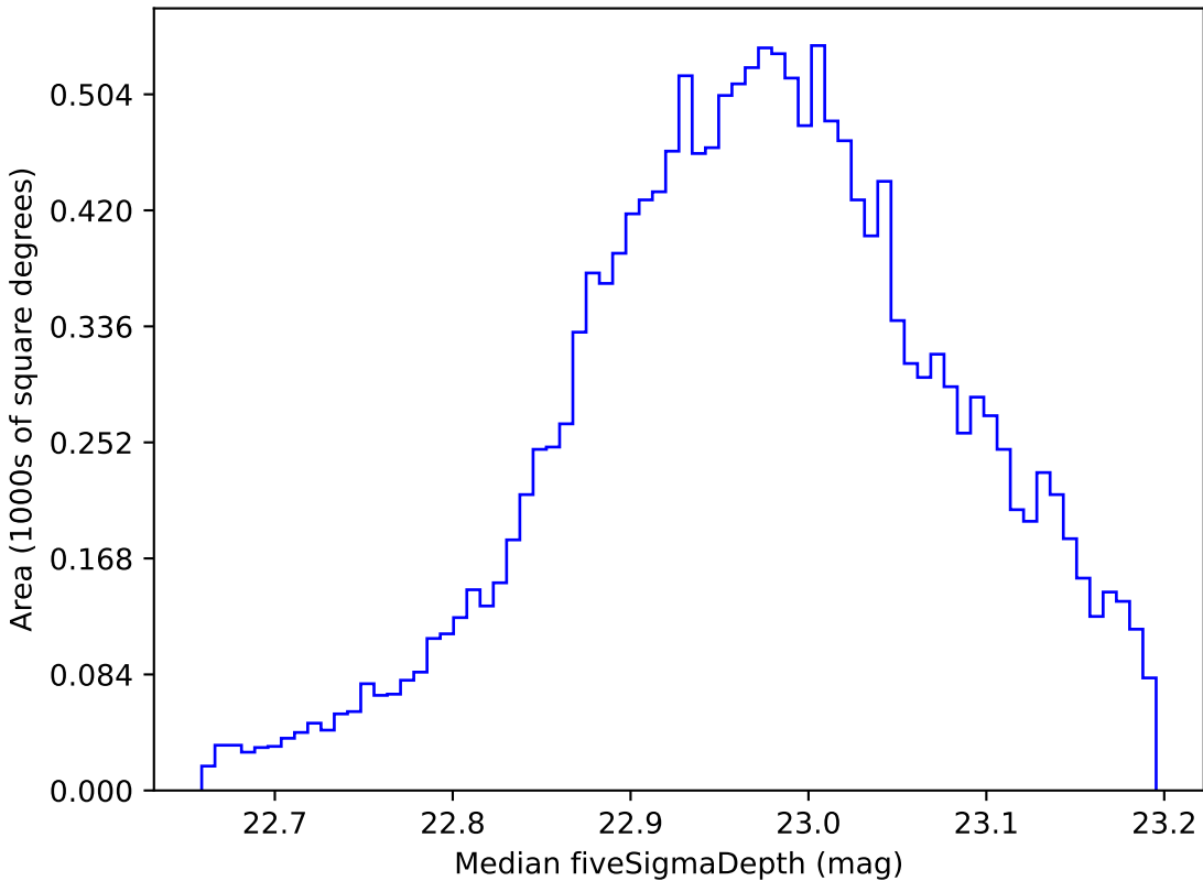
roman_v3.3_10yrs WFD z band: Median fiveSigmaDepth
