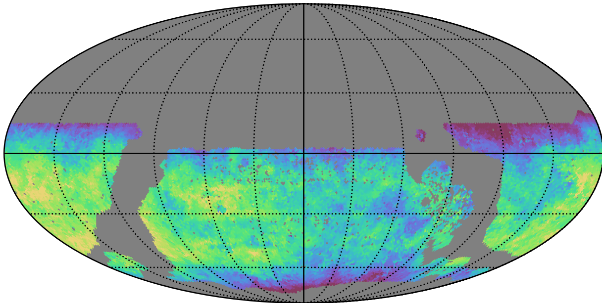
roman_v3.3_10yrs WFD u band: Median fiveSigmaDepth
