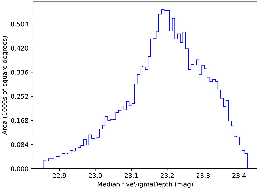
roman_v3.3_10yrs WFD u band: Median fiveSigmaDepth
