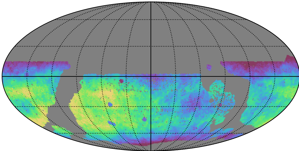
roman_v3.3_10yrs WFD r band: Median fiveSigmaDepth
