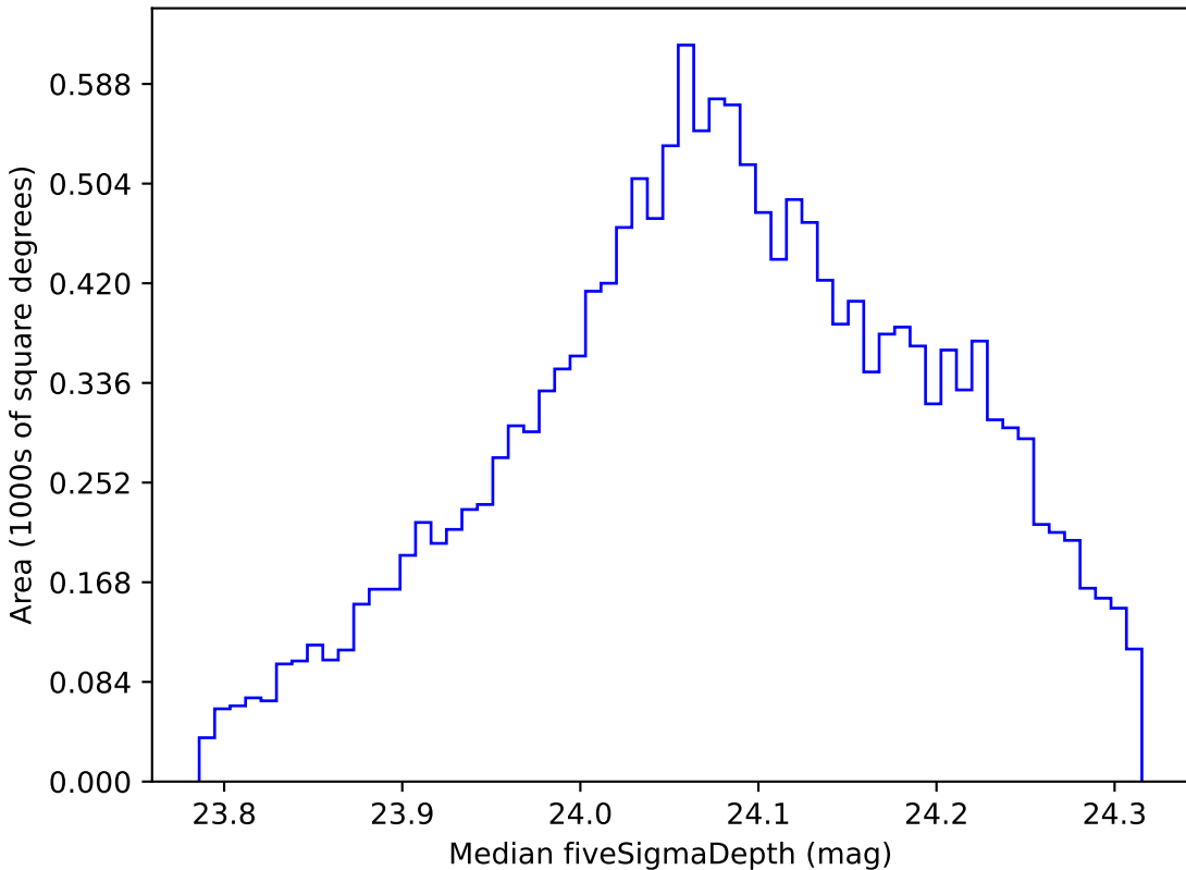
roman_v3.3_10yrs WFD r band: Median fiveSigmaDepth
