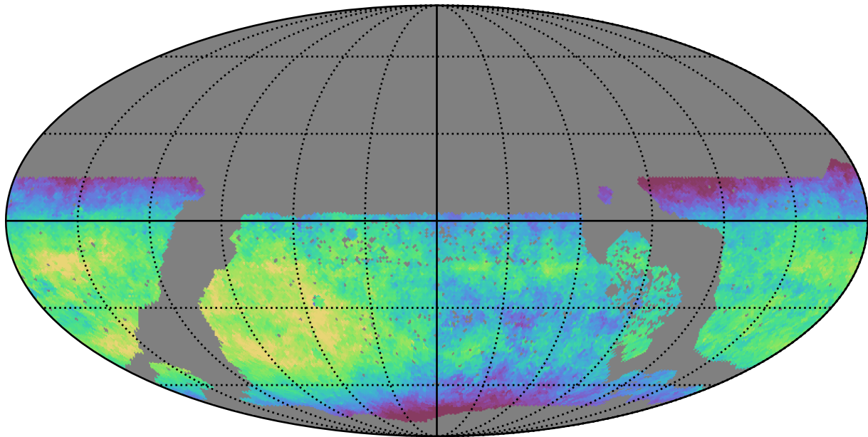
roman_v3.3_10yrs WFD i band: Median fiveSigmaDepth
