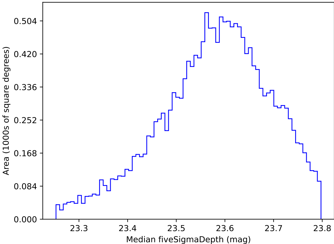
roman_v3.3_10yrs WFD i band: Median fiveSigmaDepth
