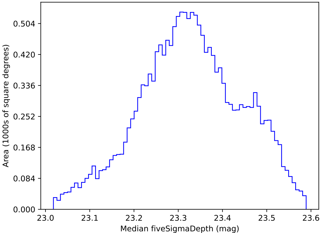
roman_v3.3_10yrs WFD all bands: Median fiveSigmaDepth
