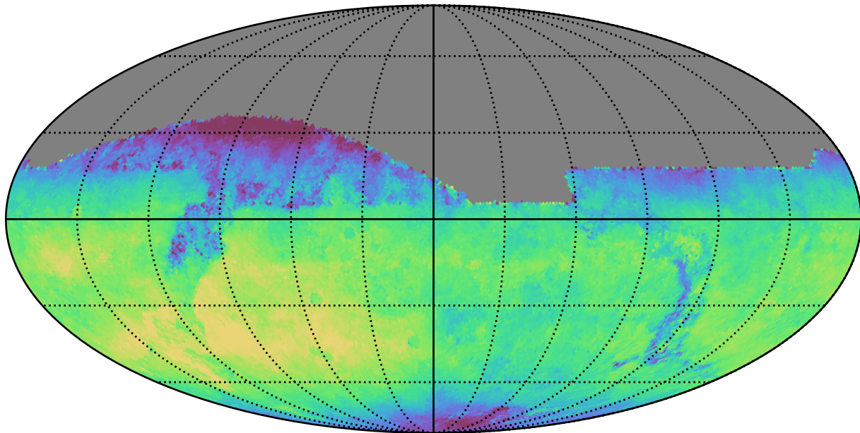
roman_v3.3_10yrs All sky z band: Median fiveSigmaDepth
