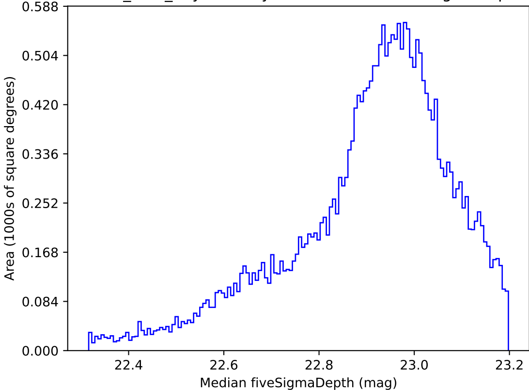
roman_v3.3_10yrs All sky z band: Median fiveSigmaDepth
