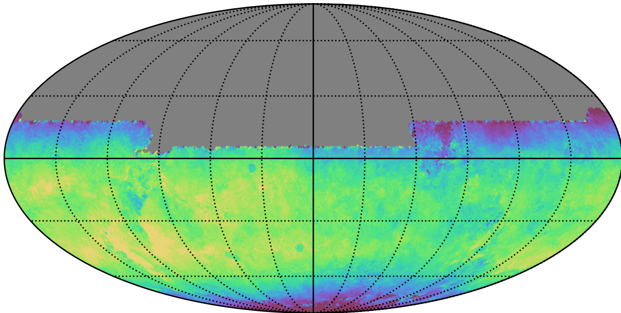
roman_v3.3_10yrs All sky y band: Median fiveSigmaDepth
