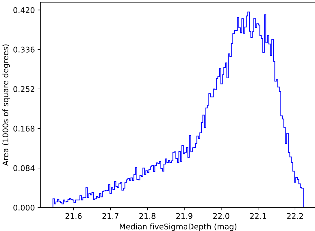
roman_v3.3_10yrs All sky y band: Median fiveSigmaDepth
