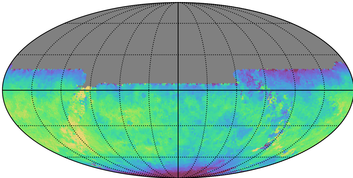
roman_v3.3_10yrs All sky u band: Median fiveSigmaDepth
