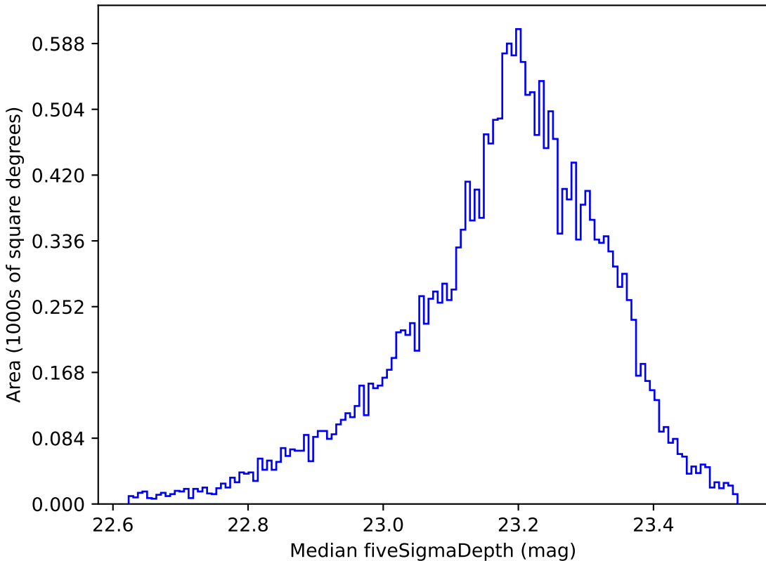
roman_v3.3_10yrs All sky u band: Median fiveSigmaDepth
