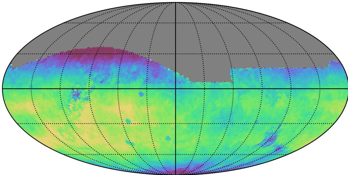
roman_v3.3_10yrs All sky r band: Median fiveSigmaDepth
