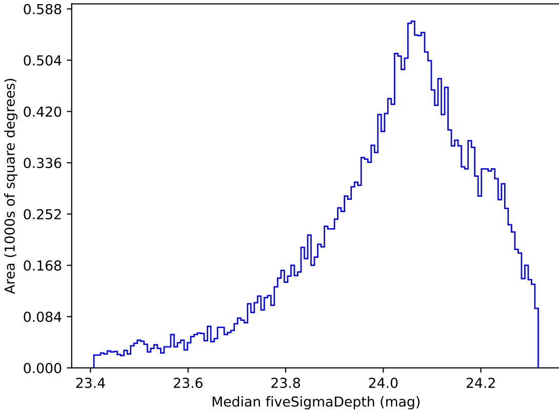
roman_v3.3_10yrs All sky r band: Median fiveSigmaDepth
