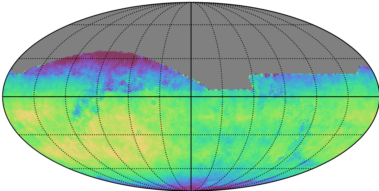
roman_v3.3_10yrs All sky i band: Median fiveSigmaDepth
