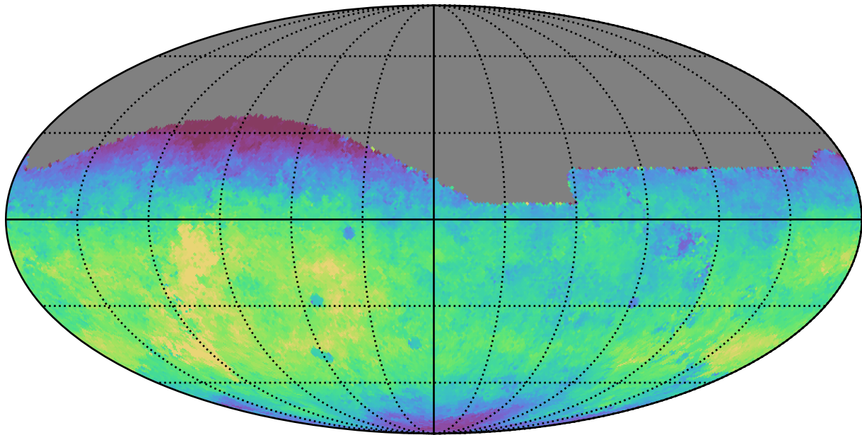
roman_v3.3_10yrs All sky g band: Median fiveSigmaDepth
