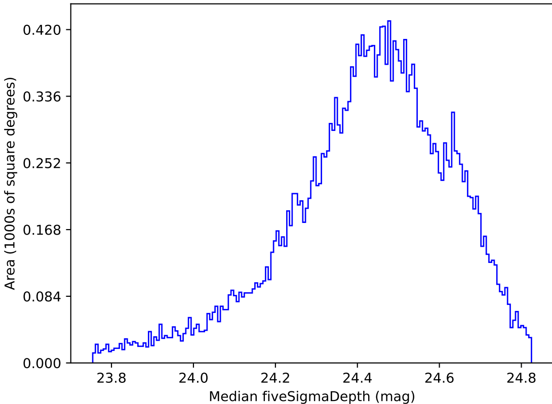
roman_v3.3_10yrs All sky g band: Median fiveSigmaDepth
