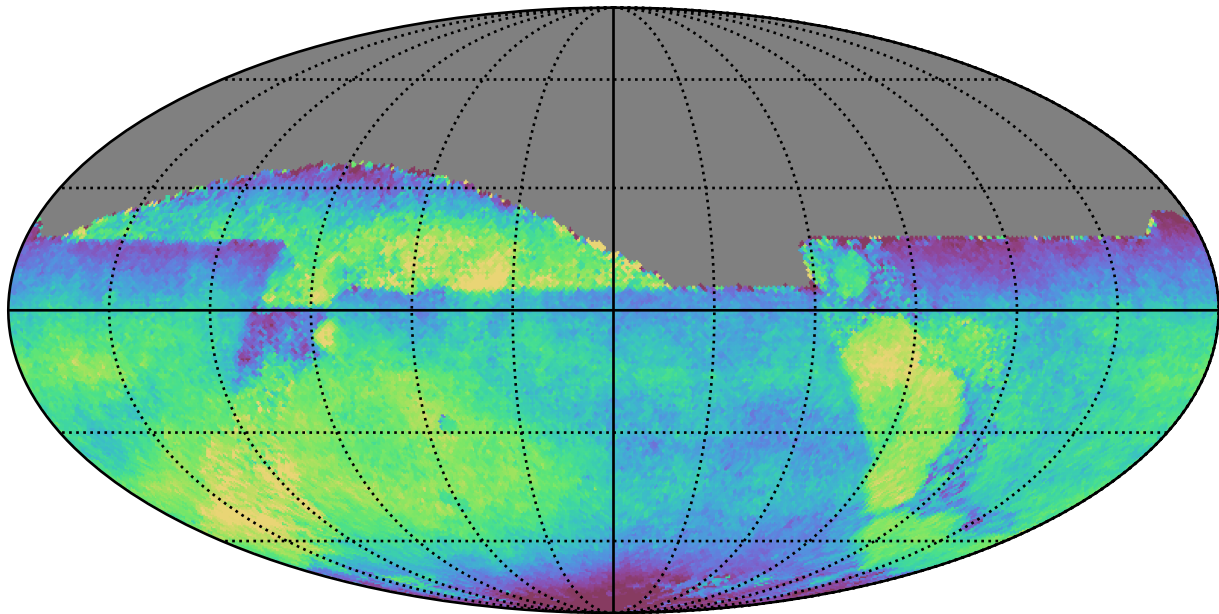
roman_v3.3_10yrs All sky all bands: Median fiveSigmaDepth
