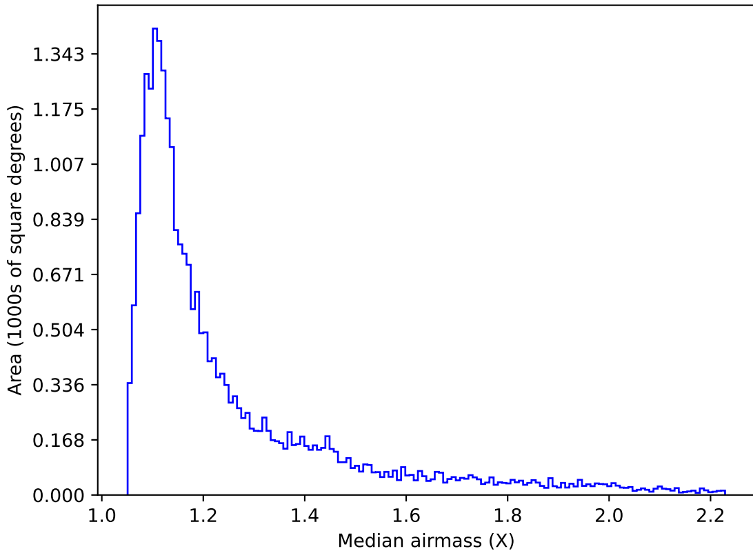
roman_v3.3_10yrs Yr 1 z band: Median airmass
