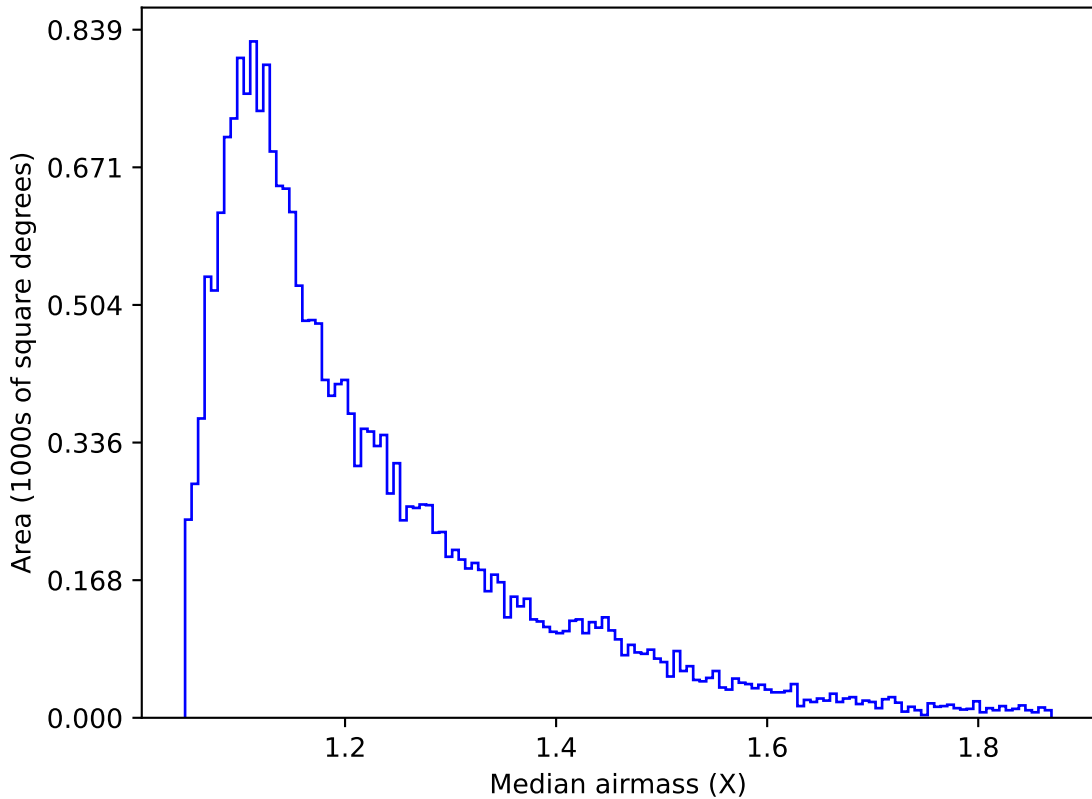
roman_v3.3_10yrs Yr 1 u band: Median airmass
