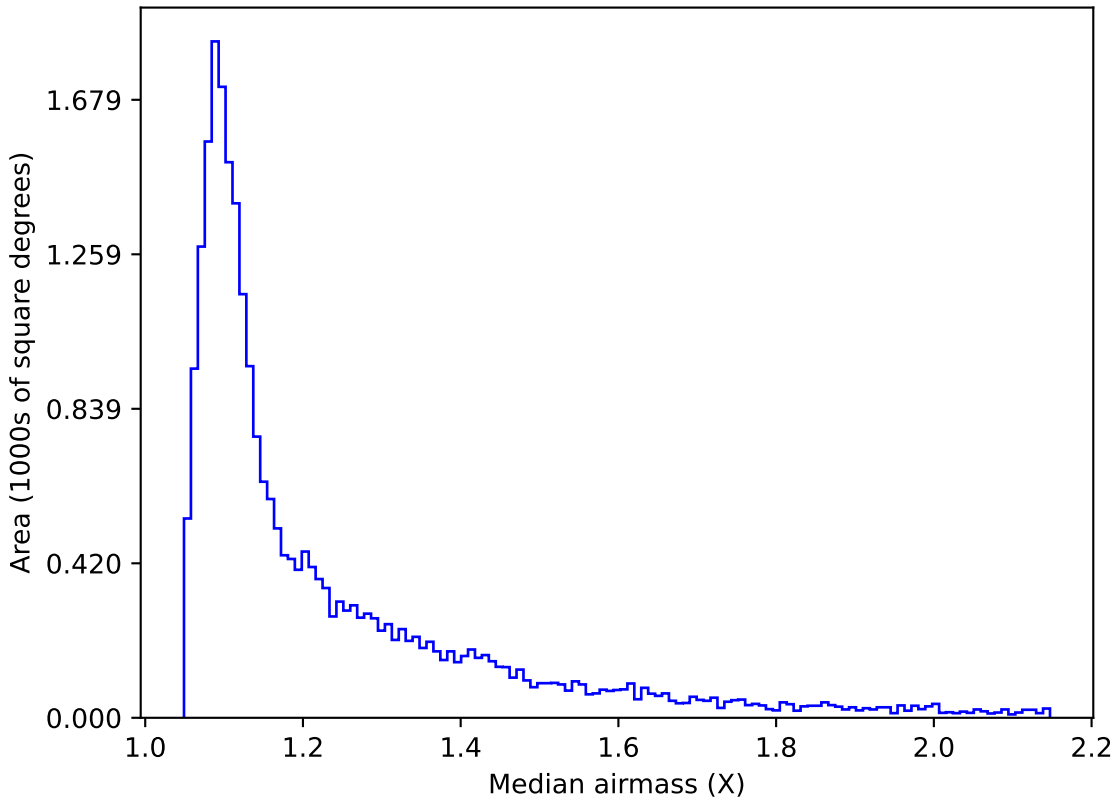
roman_v3.3_10yrs Yr 1 r band: Median airmass
