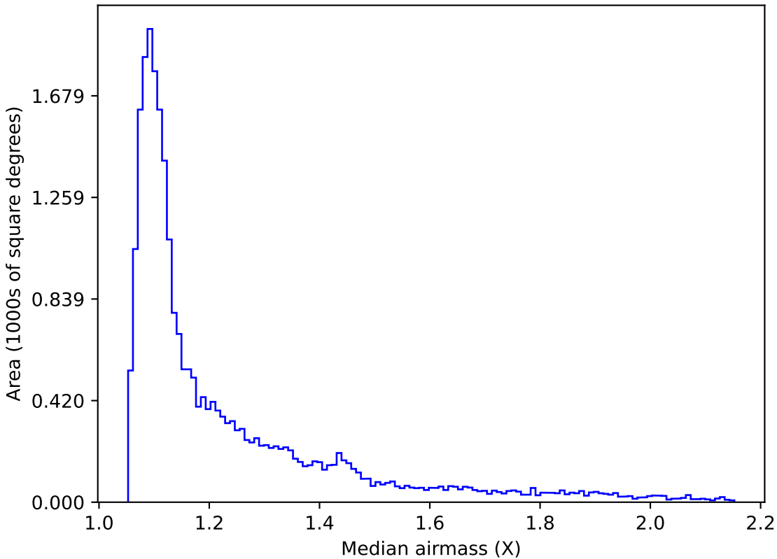
roman_v3.3_10yrs Yr 1 i band: Median airmass
