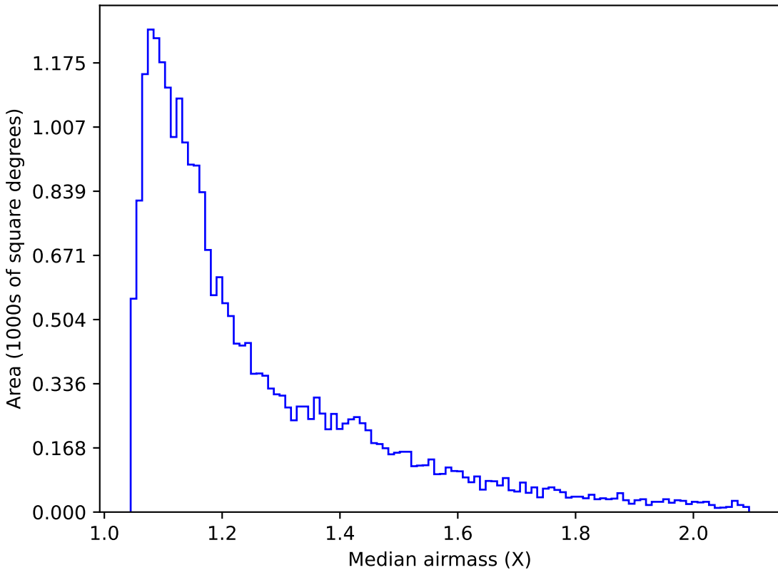
roman_v3.3_10yrs Yr 1 g band: Median airmass
