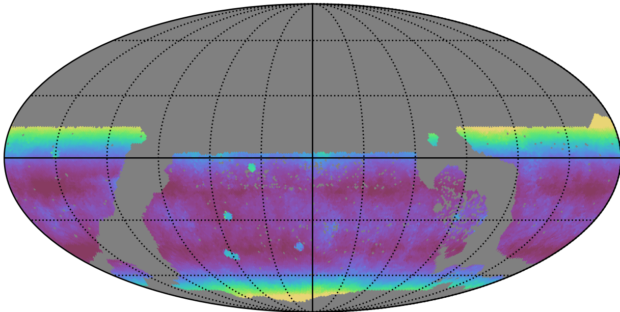
roman_v3.3_10yrs WFD z band: Median airmass
