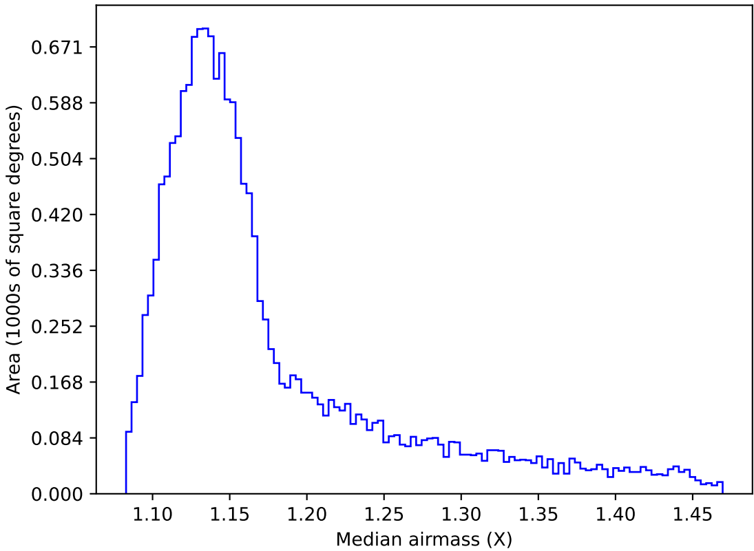
roman_v3.3_10yrs WFD z band: Median airmass
