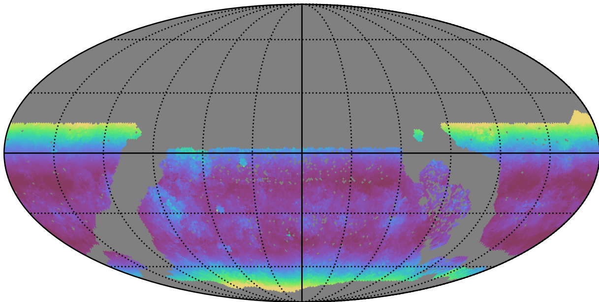
roman_v3.3_10yrs WFD u band: Median airmass
