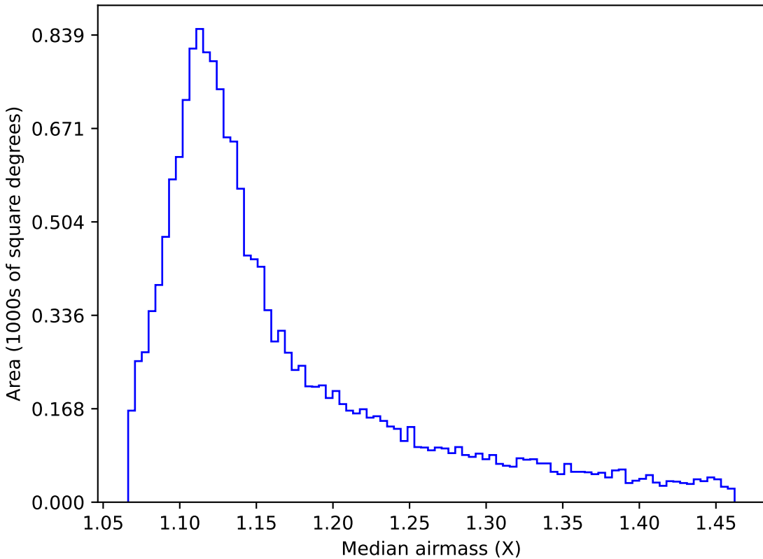
roman_v3.3_10yrs WFD u band: Median airmass
