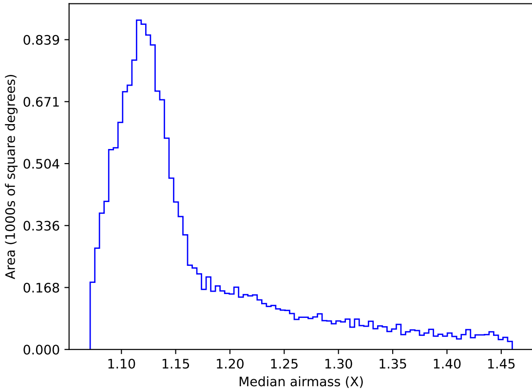
roman_v3.3_10yrs WFD r band: Median airmass
