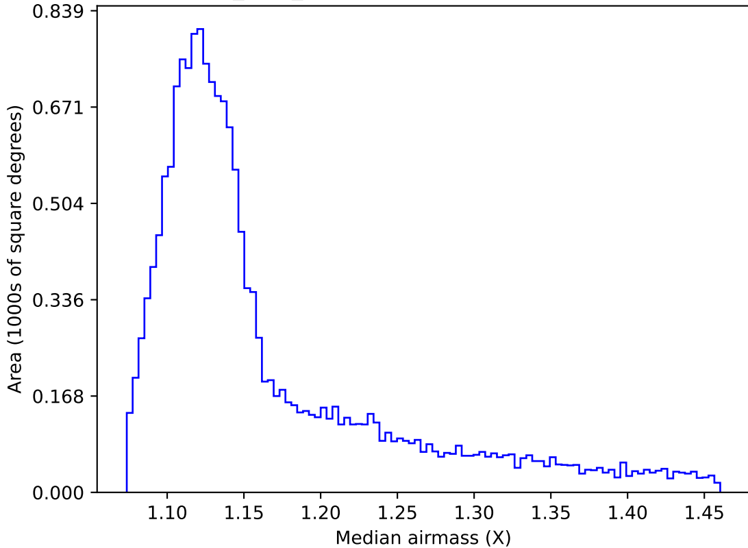
roman_v3.3_10yrs WFD i band: Median airmass
