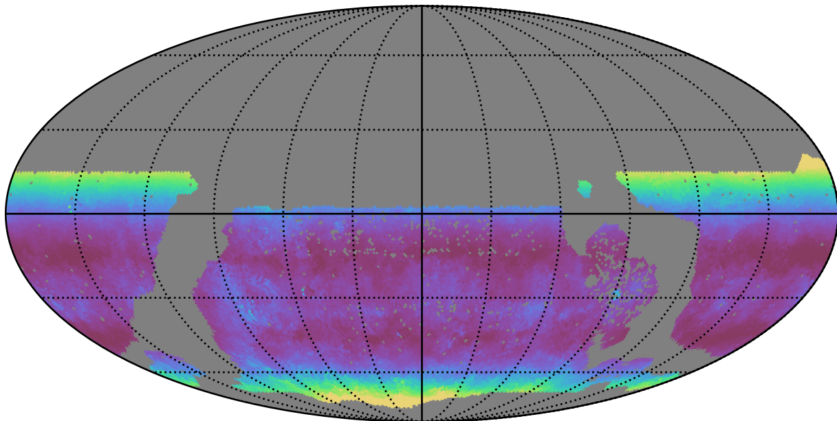
roman_v3.3_10yrs WFD g band: Median airmass
