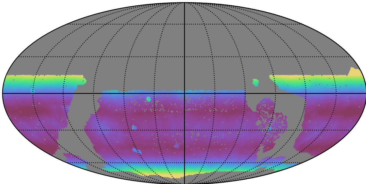
roman_v3.3_10yrs WFD all bands: Median airmass
