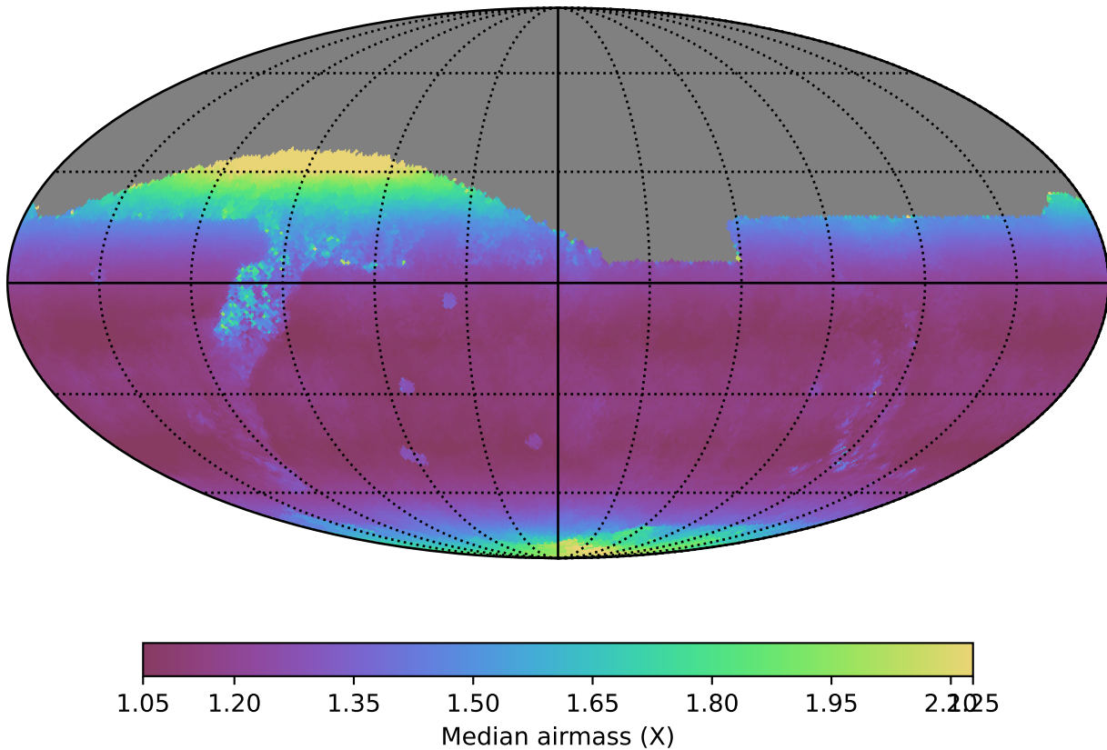
roman_v3.3_10yrs All sky z band: Median airmass
