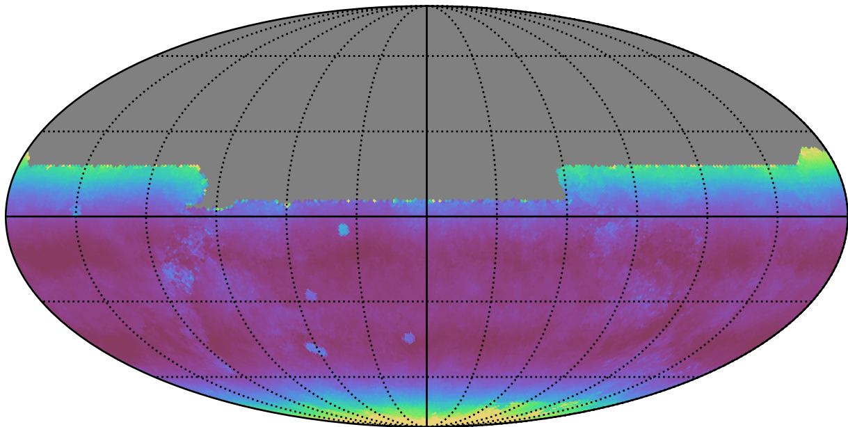
roman_v3.3_10yrs All sky y band: Median airmass
