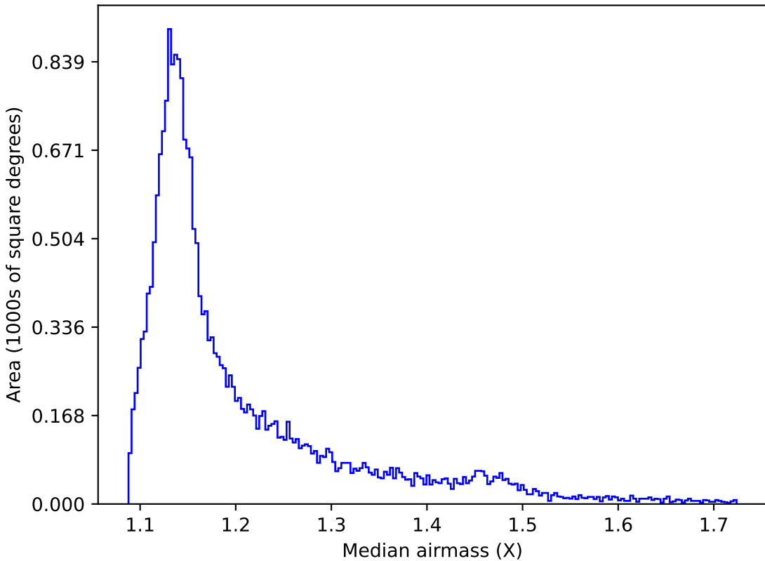
roman_v3.3_10yrs All sky y band: Median airmass
