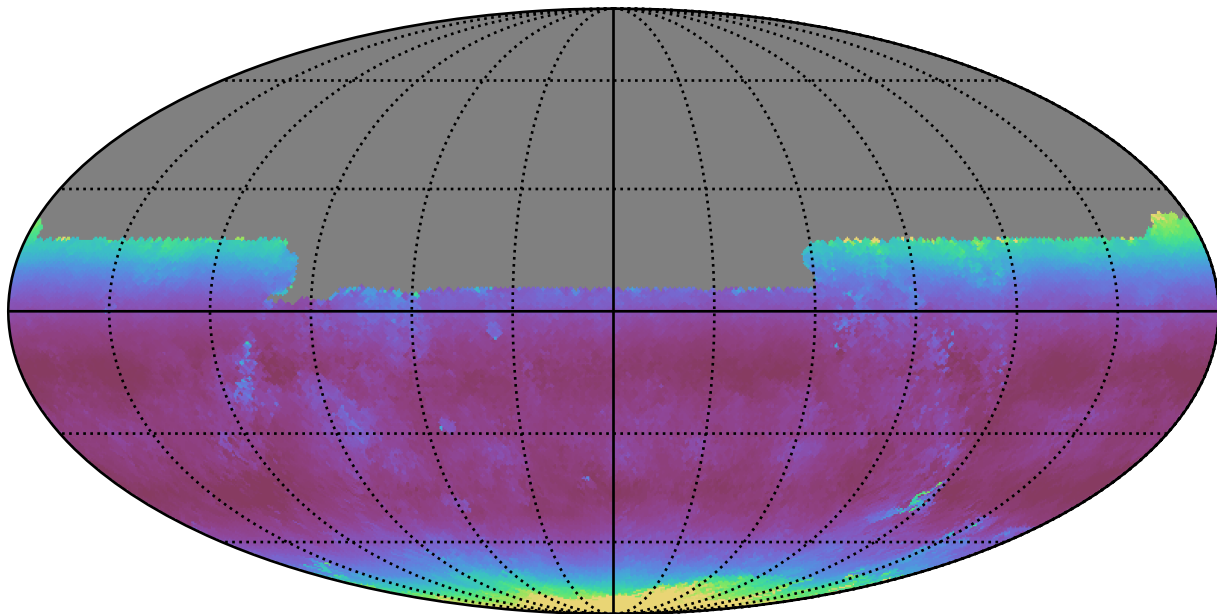
roman_v3.3_10yrs All sky u band: Median airmass
