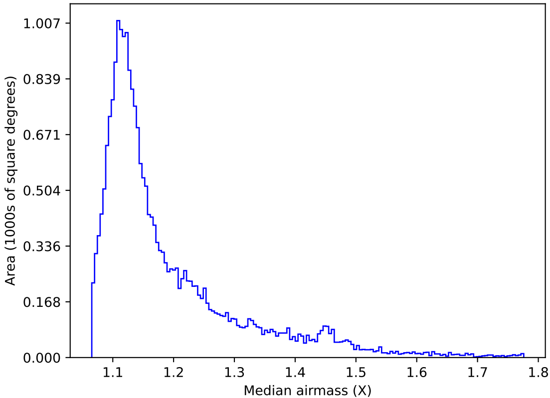
roman_v3.3_10yrs All sky u band: Median airmass
