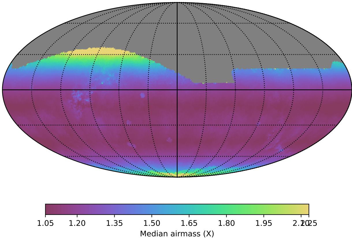
roman_v3.3_10yrs All sky r band: Median airmass
