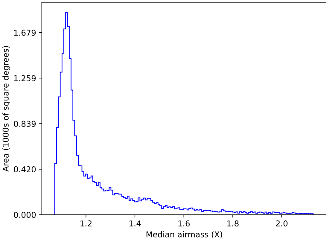
roman_v3.3_10yrs All sky r band: Median airmass
