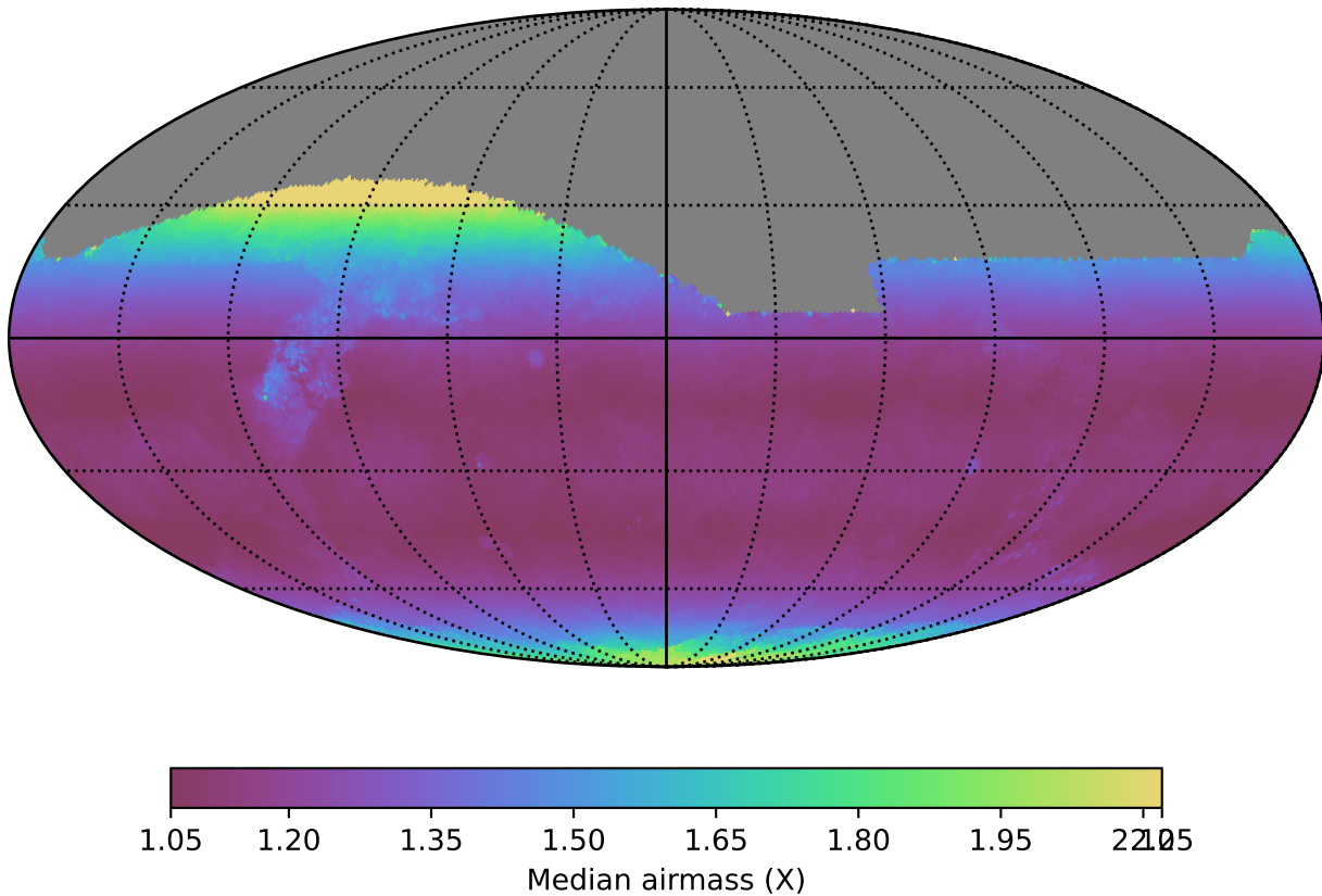
roman_v3.3_10yrs All sky i band: Median airmass
