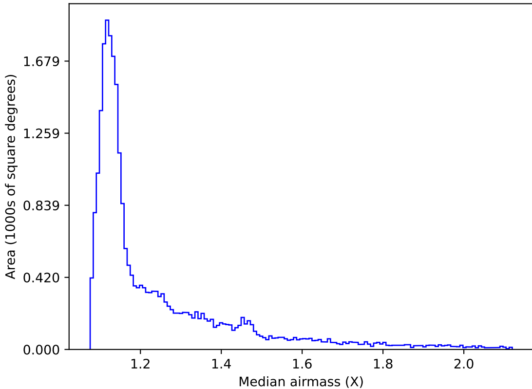
roman_v3.3_10yrs All sky i band: Median airmass
